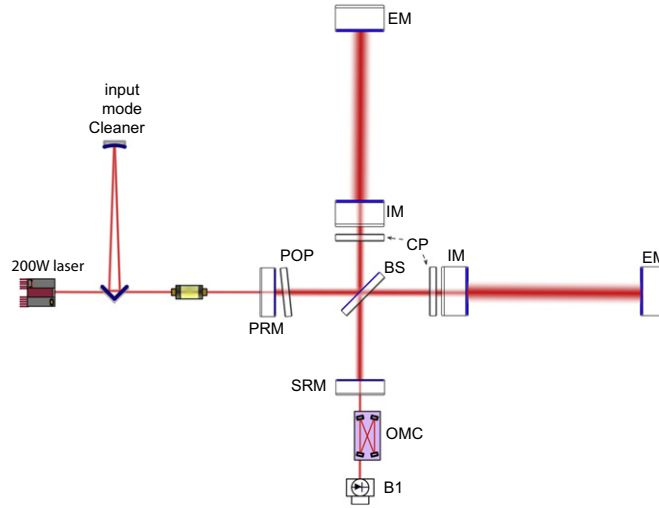
Figure 3. Simplified optical layout of the AdV ITF. Each 3 km long arm cavity is formed by an IM and an EM. The recycling cavities at the center of the ITF are 12 meters long and are formed by the PRM, the SRM and the two IM.
