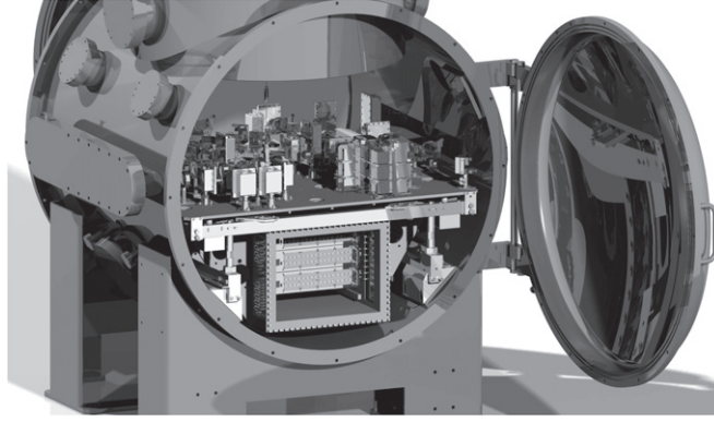
Figure 20. A 3D drawing of the new suspended bench inside its vacuum chamber.
